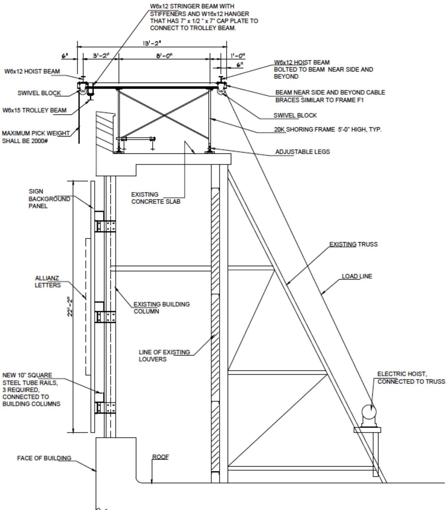
SECTION VIEW AT TOP OF BUILDING, SHOWING HOISTING SYSTEM
