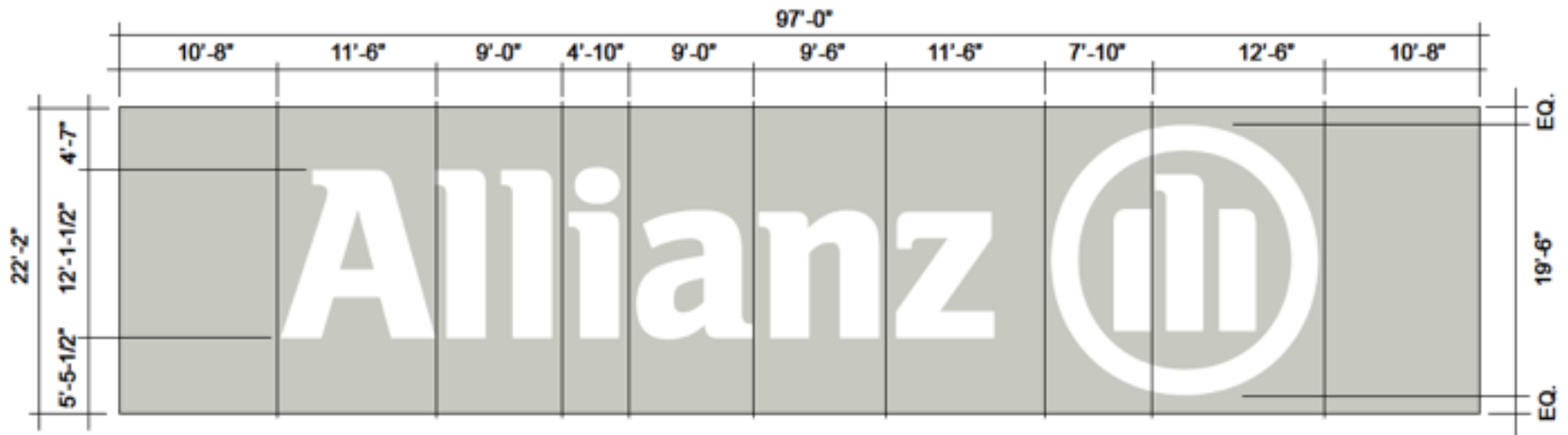
VERTICAL SECTIONS DETAIL - SCALE: 1/8" = 1'-0"
